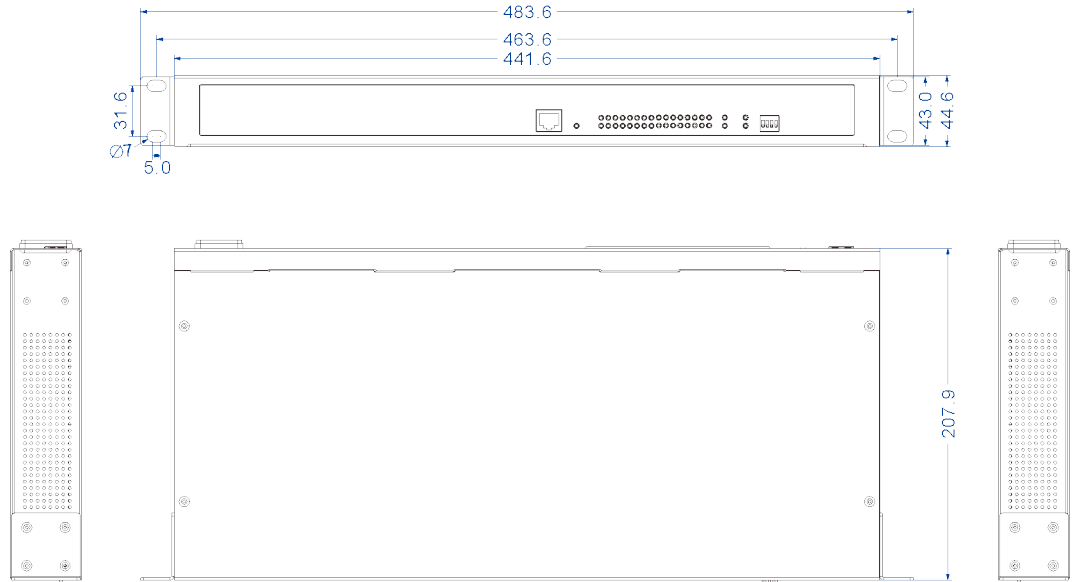
NP3016T-16D(232) & NP3016T-16D(3IN1)
